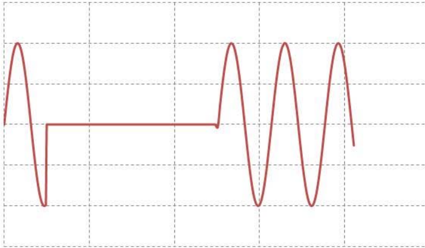
Figure 6. Voltage interruption
